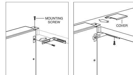
Countertop mounting.
