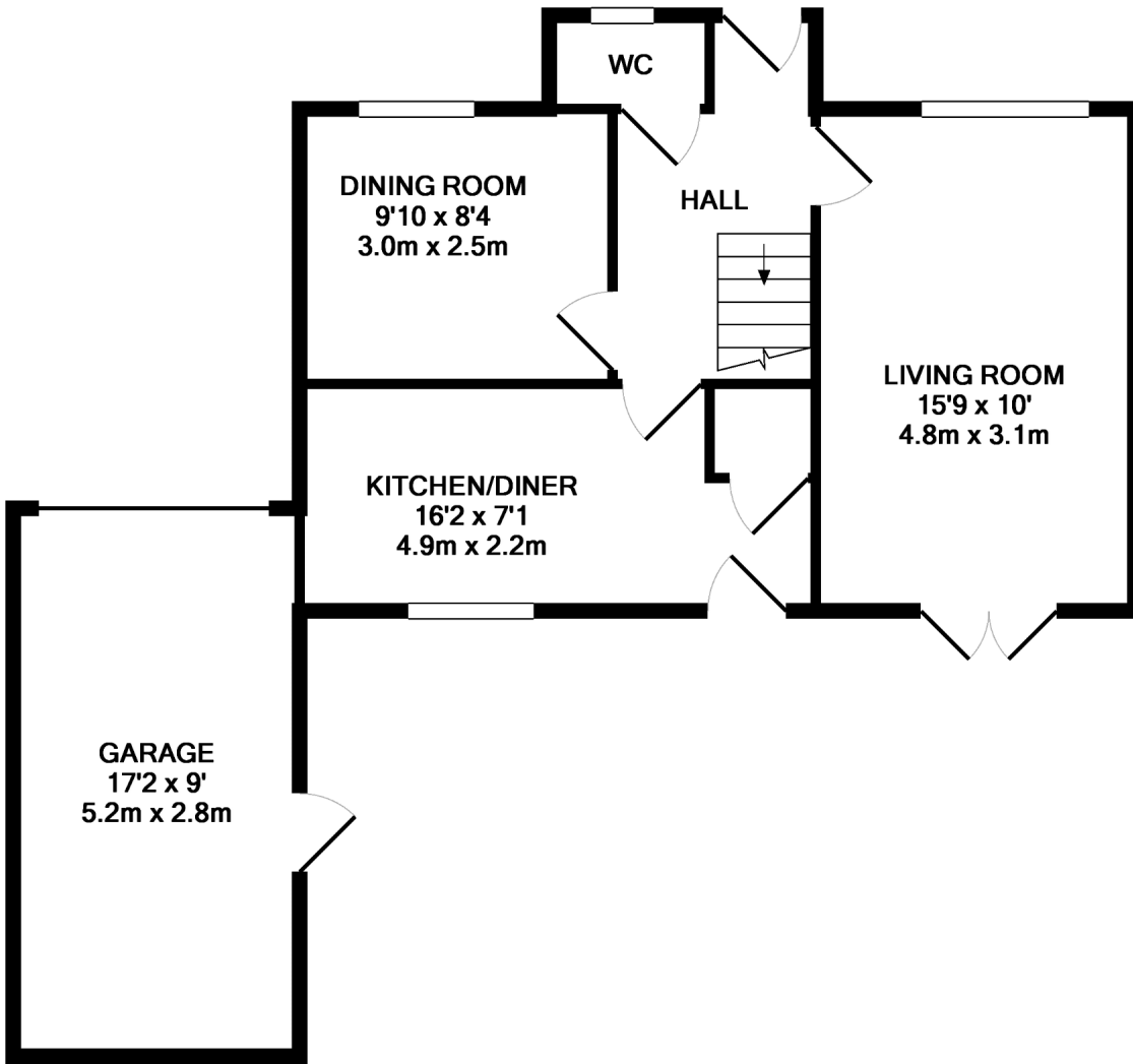
GROUND FLOOR APPROX. FLOOR AREA 592 SQ.FT. (55.0 SQ.M.)
