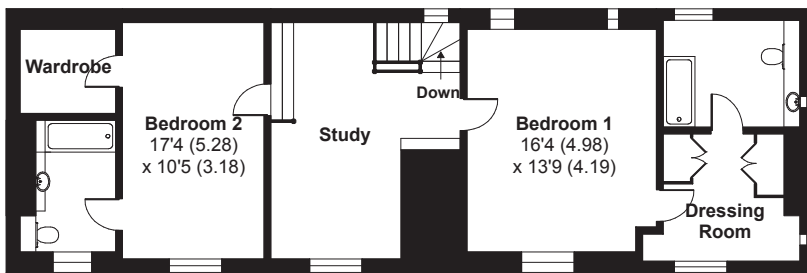
FIRST FLOOR 2
