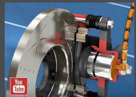
HOW CAR BRAKES WORK BENDIX BRAKES
