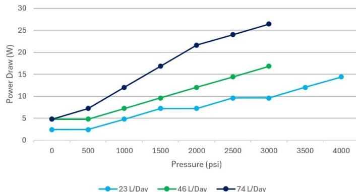
Average Power Draw of 1/4"- TR5100 Single-Sided 2-Head Pump
