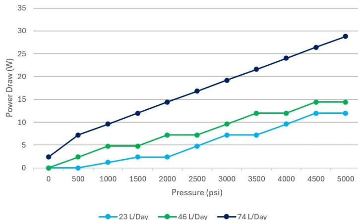
Average Power Draw of 1/2" - TR5100 Dual-Sided 2-Head Pump
