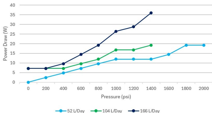
Average Power Draw of 3/8"- TR5100 Single-Sided 2-Head Pump
