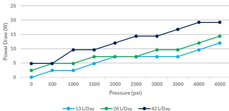
Average Power Draw of 3/16"- TR5100 Single-Sided 2-Head Pump
