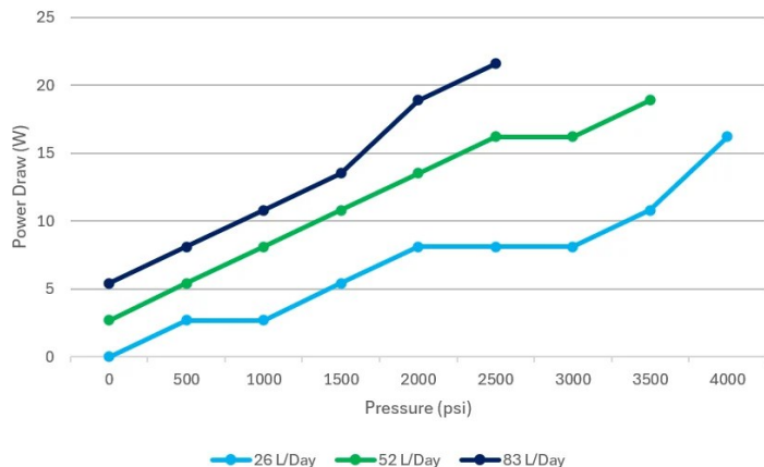
Average Power Draw of 3/8"- TR5100 Single-Sided 1-Head Pump
