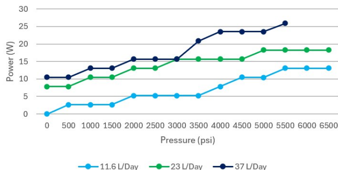
Average Power Draw of 1/4"- TR5100 Single-Sided 1-Head Pump
