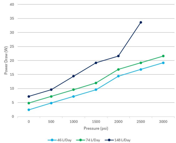
Average Power Draw of 1/2"- TR5100 Dual-Sided 4-Head Pump
