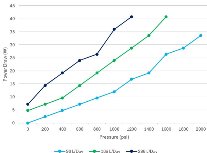
Average Power Draw of 1/2" - TR5100 Dual-Sided 2-Head Pump
