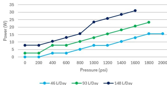
Average Power Draw of 1/2"- TR5100 Single-Sided 1-Head Pump
