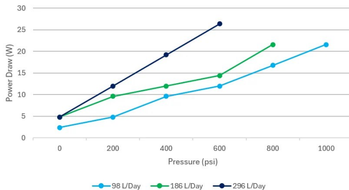
Average Power Draw of 1/2"- TR5100 Single-Sided 2-Head Pump
