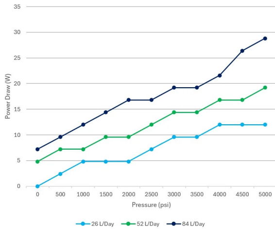
Average Power Draw of 3/16"- TR5100 Dual-Sided 4-Head Pump
