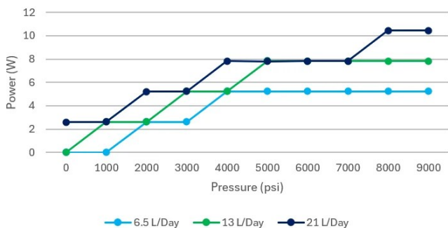
Average Power Draw of 3/16"- TR5100 Single-Sided 1-Head Pump
