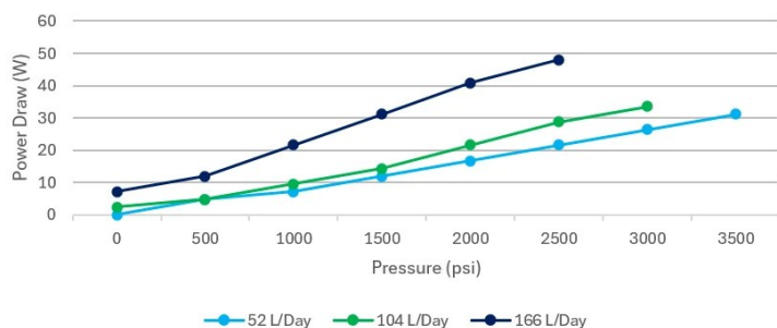
Average Power Draw of 3/8" - TR5100 Dual-Sided 2-Head Pump
