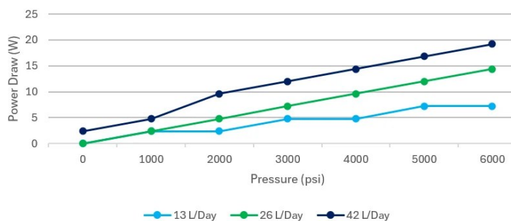
Average Power Draw of 3/16" - TR5100 Dual-Sided 2-Head Pump
