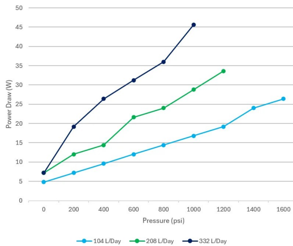
Average Power Draw of 3/8"- TR5100 Dual-Sided 4-Head Pump
