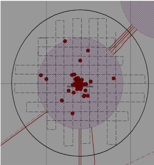
Blackbird Subsea Facilities (57° 50.964'N, 000° 37.128'W)
