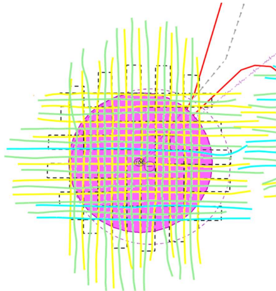
Blackbird Water Injection Well (57° 50.860'N, 000° 38.674'W)
