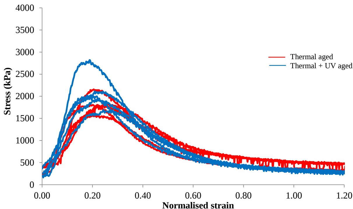
(c) Slab C results – UV & thermal aged vs. thermal aged samples
