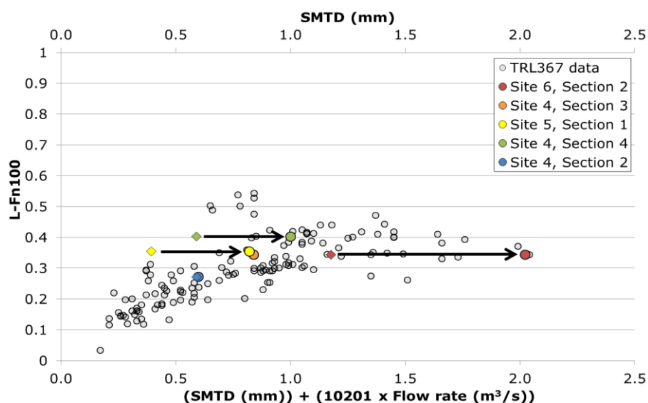
Figure 4-1 Texture depth, permeability and high speed friction of selected specimens
