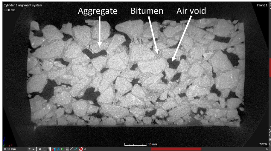
Figure 4-4 Front panel (bottom left) from Figure 4-3
