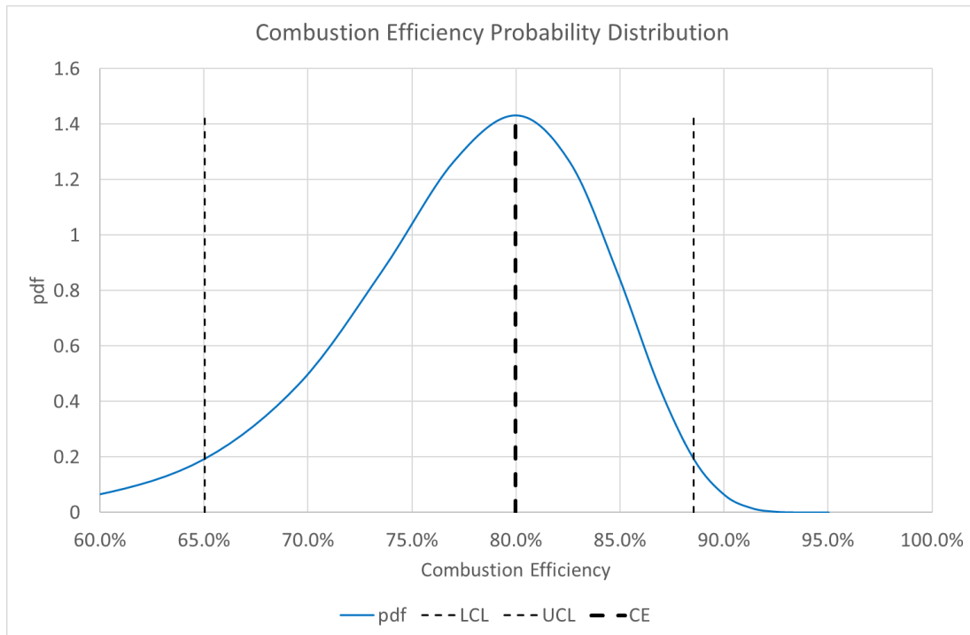
Figure 12 CE Uncertainty Probability Distribution for Base Case, Wind Speed increased to 25.8 m/s, UoA Coefficient Covariance Excluded
