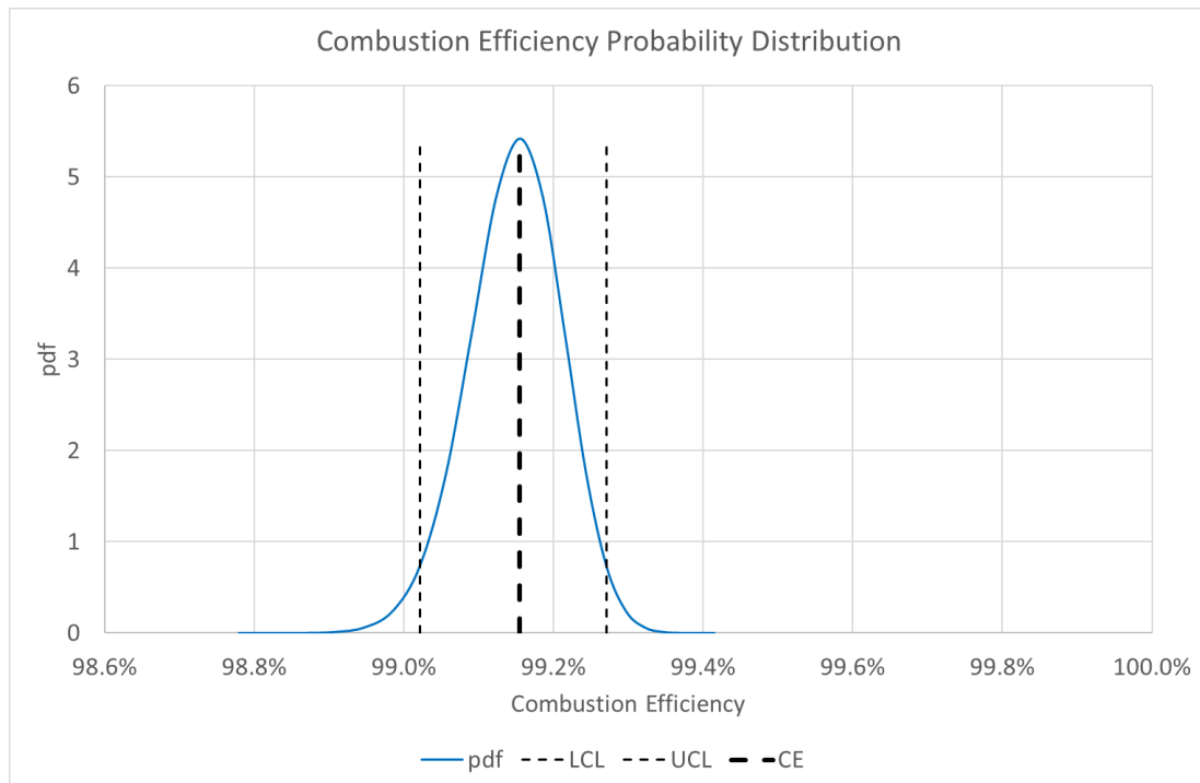
Figure 10 CE Uncertainty Probability Distribution for Base Case, Wind Speed 10 m/s
