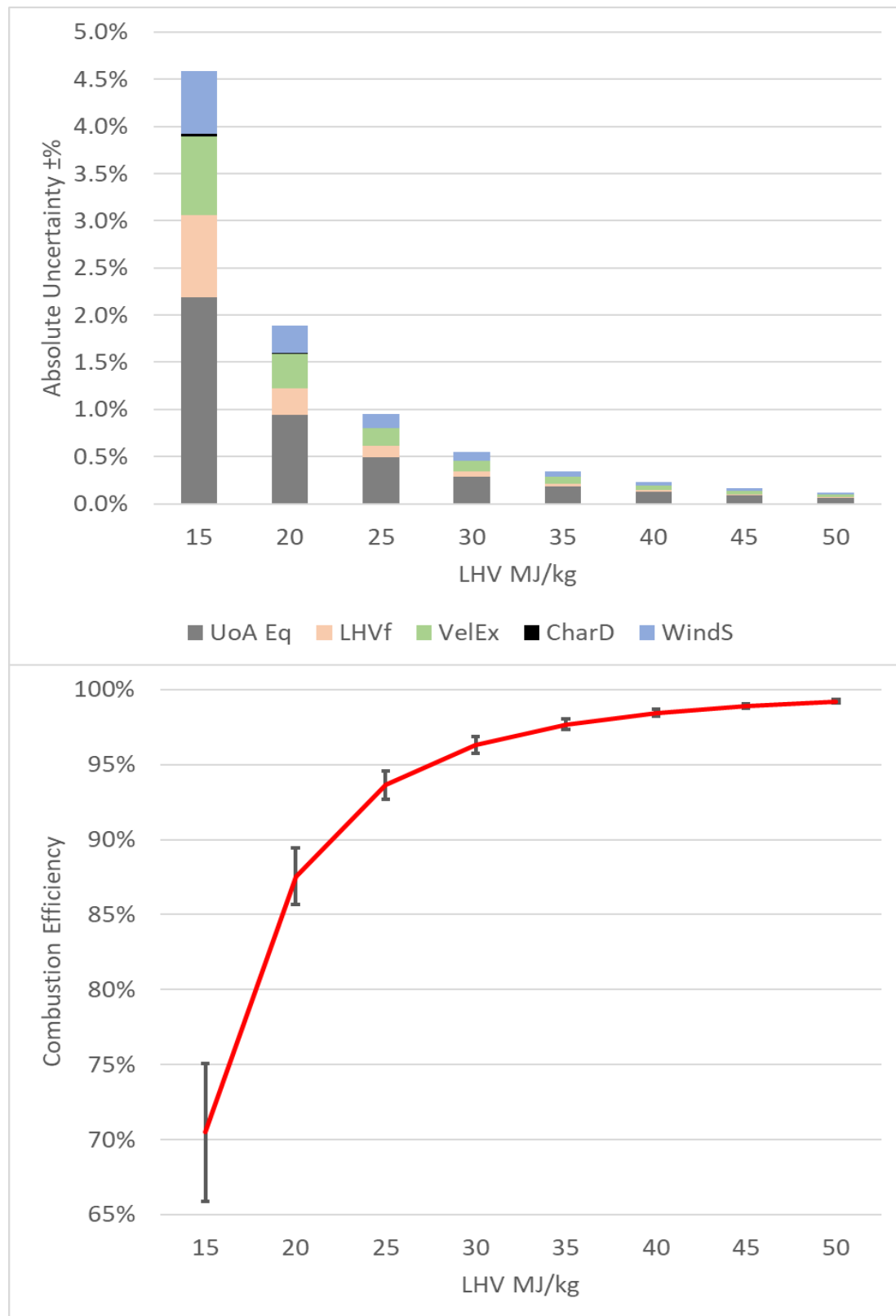
Figure 13 CE and Associated Uncertainties, LHV Sensitivity
