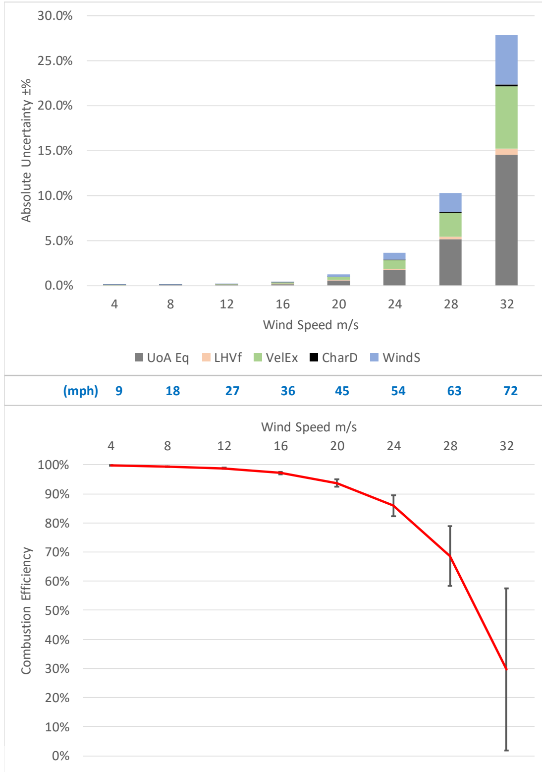
Figure 14 CE and Associated Uncertainties, Wind Speed Sensitivity
