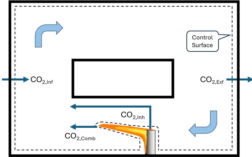
Figure 4 Schematic of a flare burning in a closed loop wind tunnel
