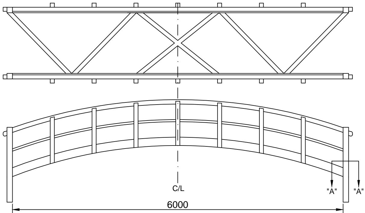
CROSS BRACING - OVER 6M (20 FOOT) SPAN
