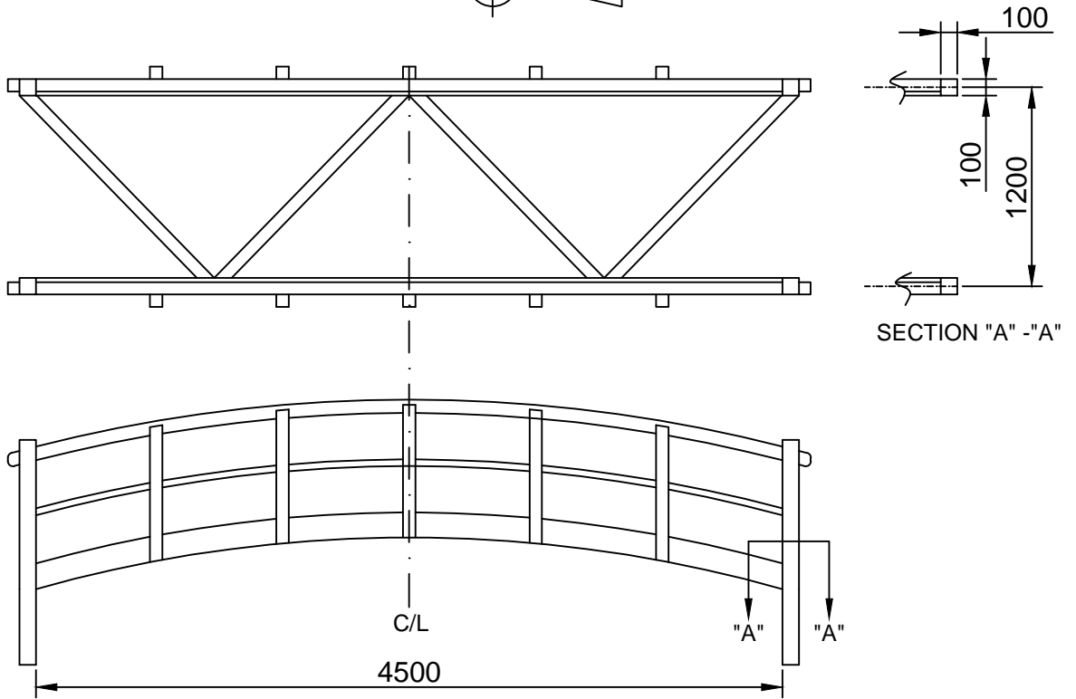
CROSS BRACING - 4.5M (15 FOOT) TO 6M (20 FOOT) SPAN
